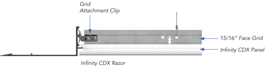
Infinity CDX Razor Edge with Grid and Rockfon CDX Edge Tile
