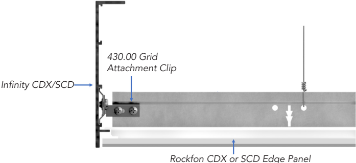
Infinity CDX Installation with Grid and Rockfon CDX Edge Tile
