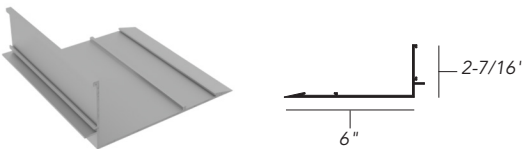
Infinity CDX Razor
